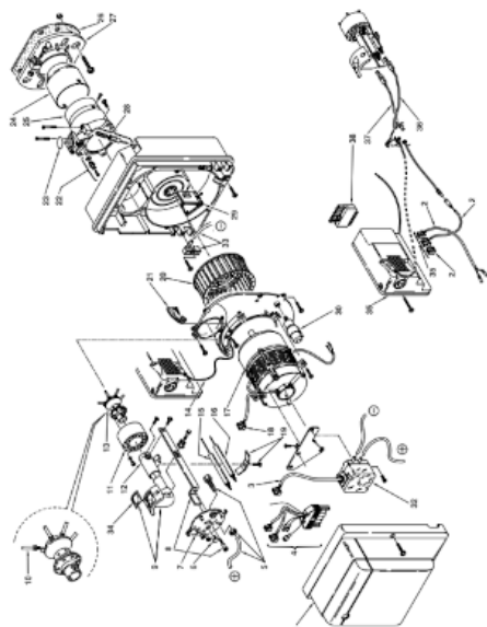
Parts for the RIELLO gas burner
